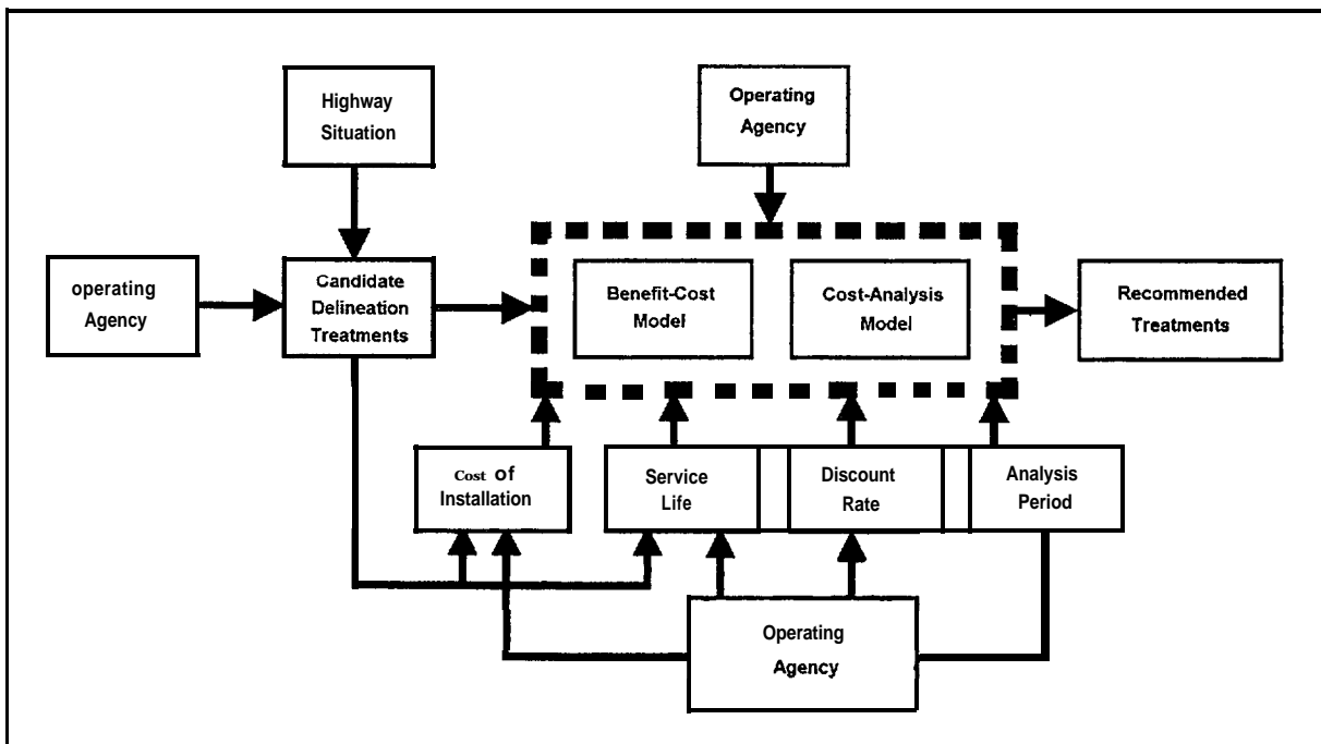
Figure 93. Schematic representation of "Benefit-Cost" and "Cost-Analysis" model
