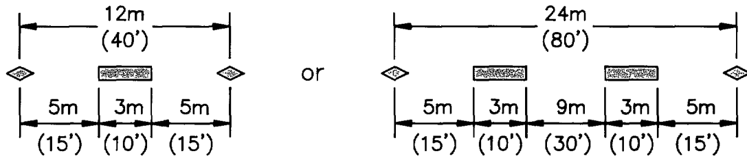
b) Combination RPM/Stripe System (2-La, 2-Way)
