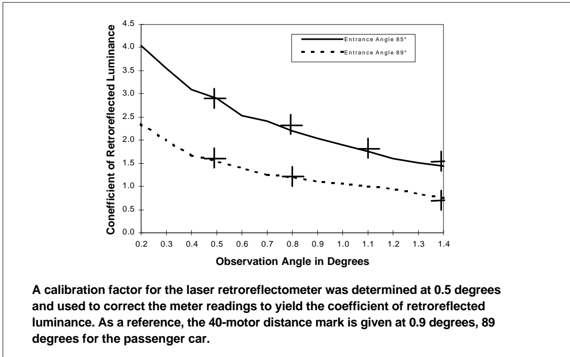
Figure 92. Retroreflection of pavement marking tape as a function of observation angle and two entrance angles
