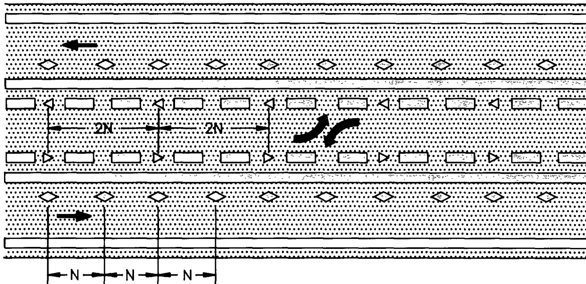
a) Center Lane of Three-Lane Road
