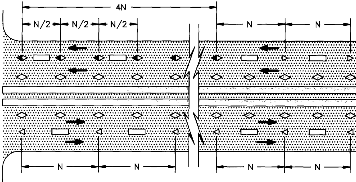
c) Four Lanes, Two-Way Roadway
