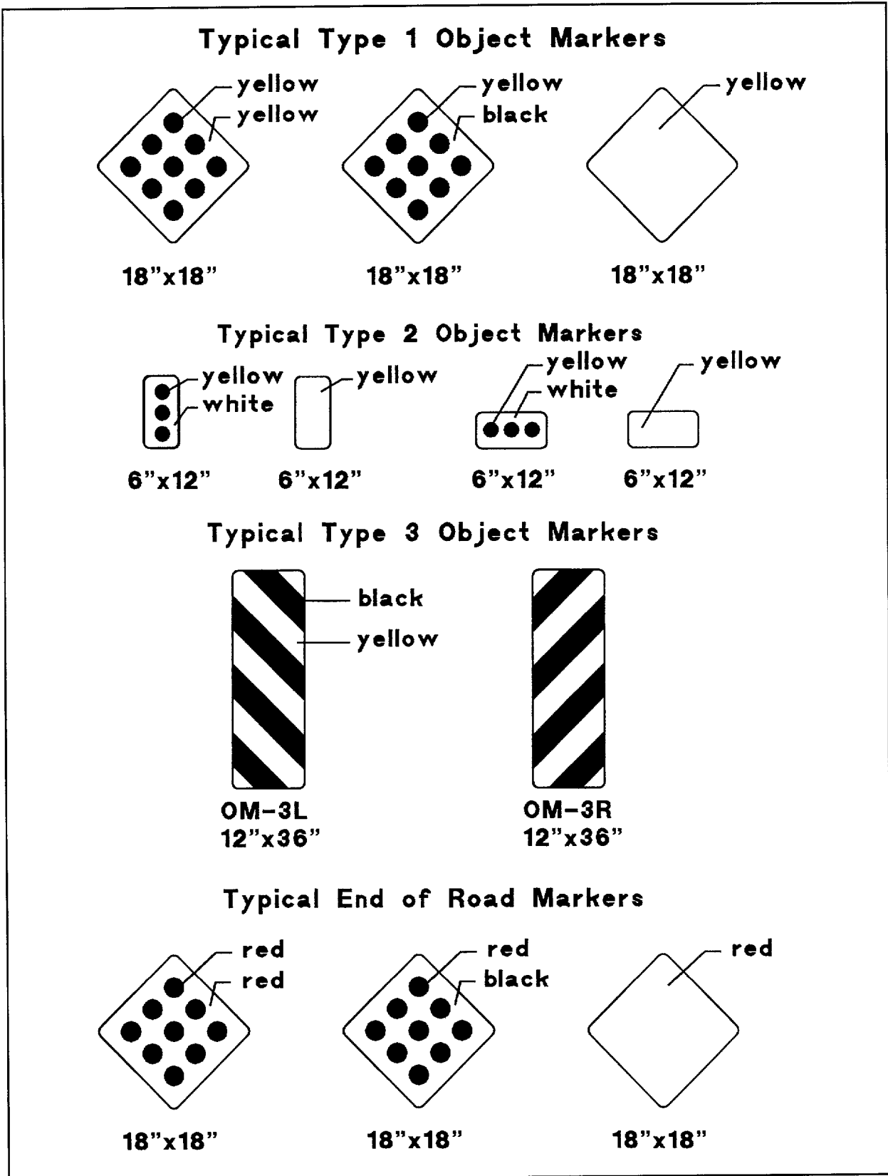
Figure 62. Object markers
