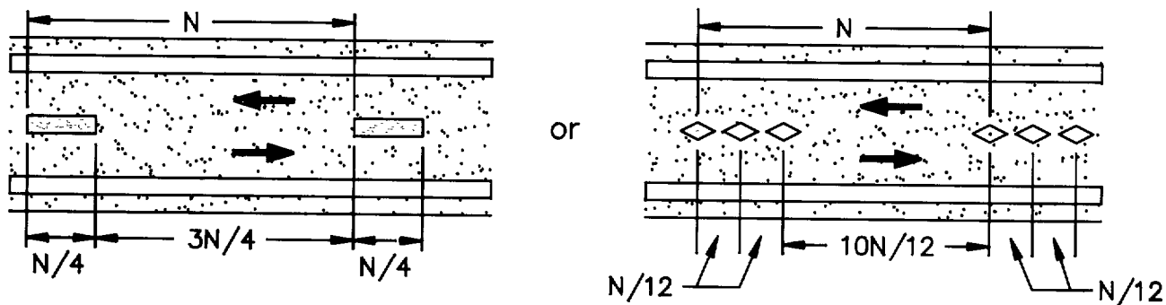
c) Two-Lane, Two-Way Road (Over 14 days)**
