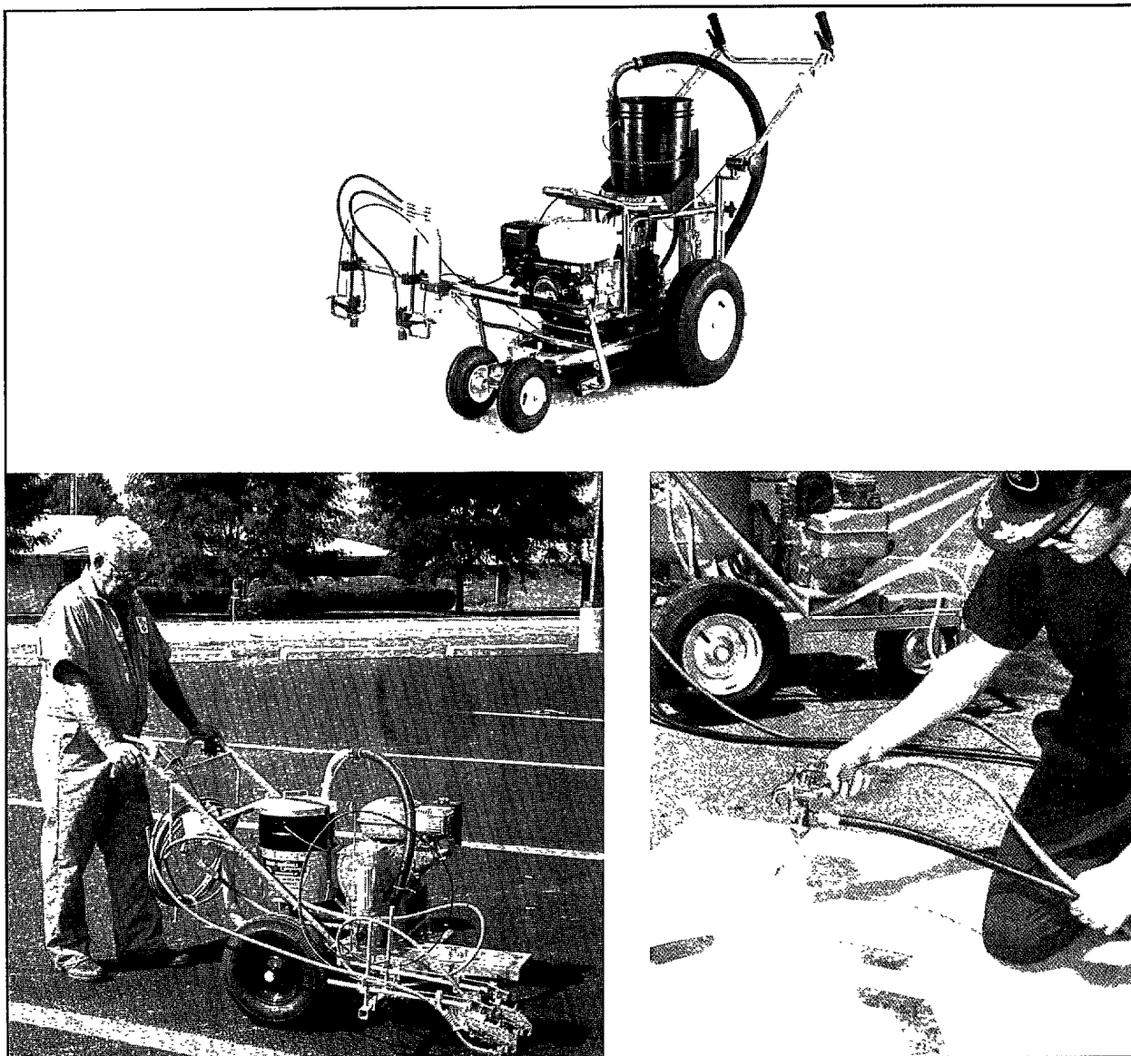
Figure 21. Small paint application units
