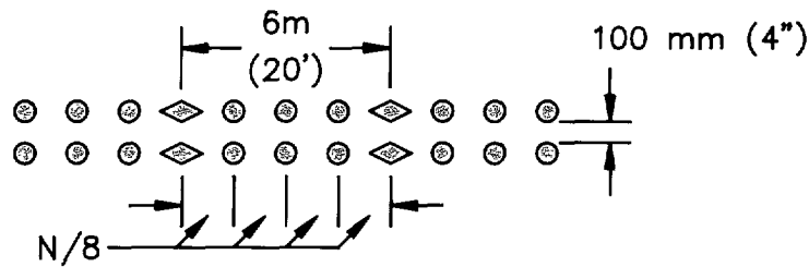
c) RPM System (Multi-La, 2-Way)
