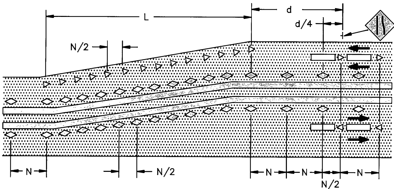
b) Four Lanes to Two-Lane Road - Left
