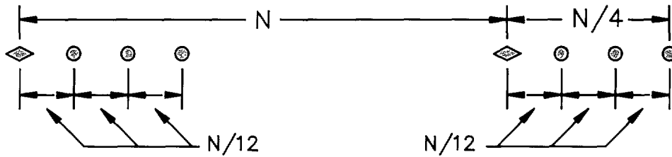
a) RPM System (2-La, 2-Way)
