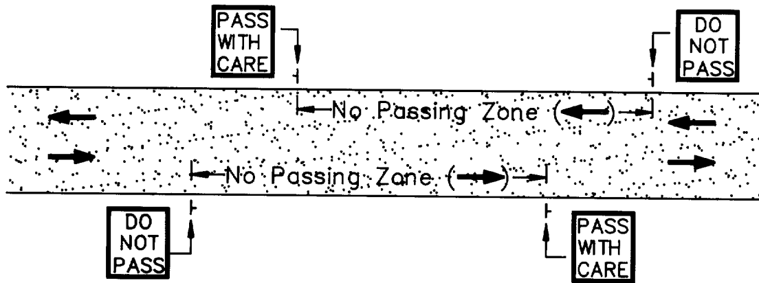
a) Two-Lane/Two-Way Road (3 days or less)*
