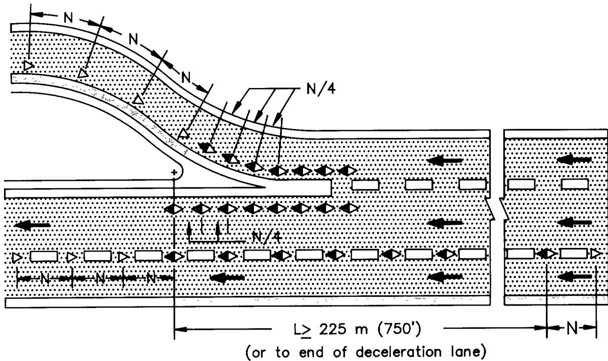
a) Exit Ramp
