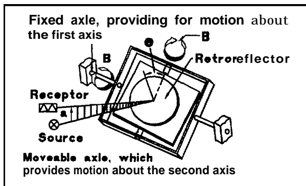
Figure 15. Retroreflection test geometry
