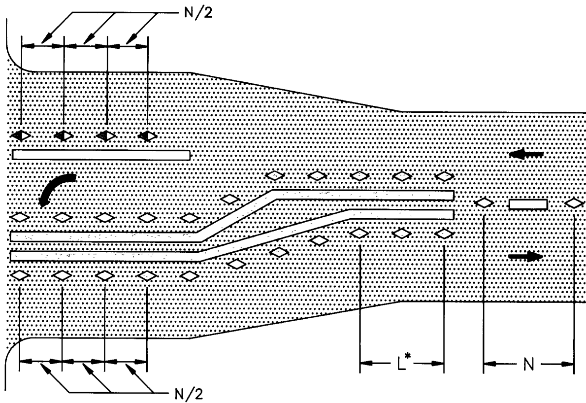
c) Protected Left-Turn
