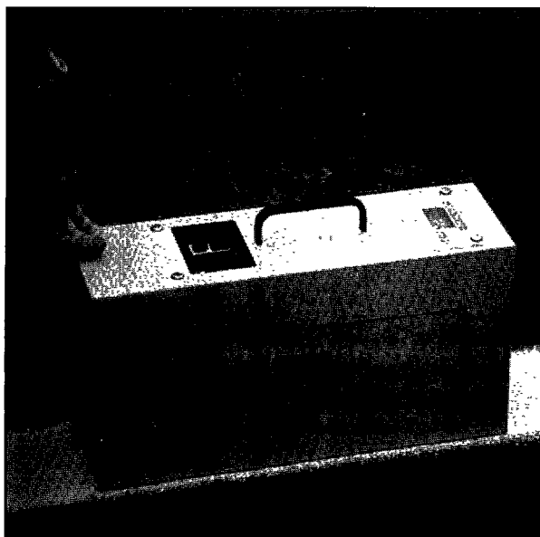
Figure 89. Mirolux 12 retroreflectometer
