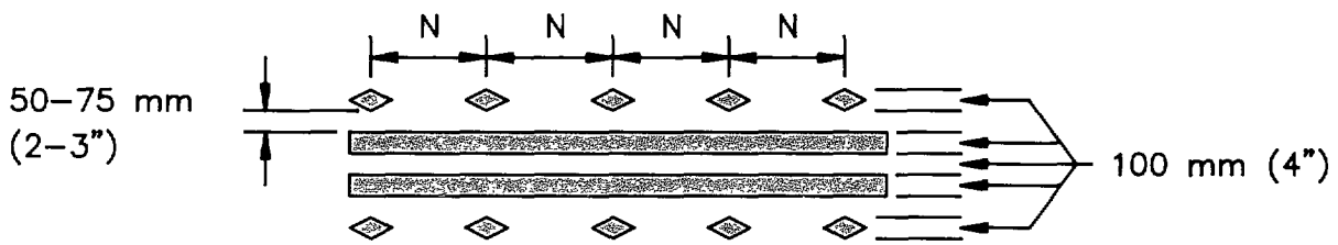
d) Combination RPM/Stripe System (Multi-La, 2-Way)
