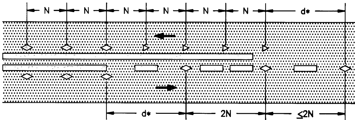
b) No Passing Zone
