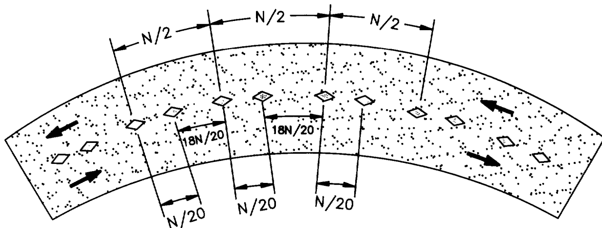
e) Two-Lane, Two-Way Road with Severe curvature (14 Days or Less), RPM Centerline**
