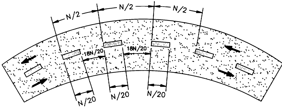
d) Two-Lane, Two-Way Road with Severe curvature (14 Days or Less), Stripe Centerline**
