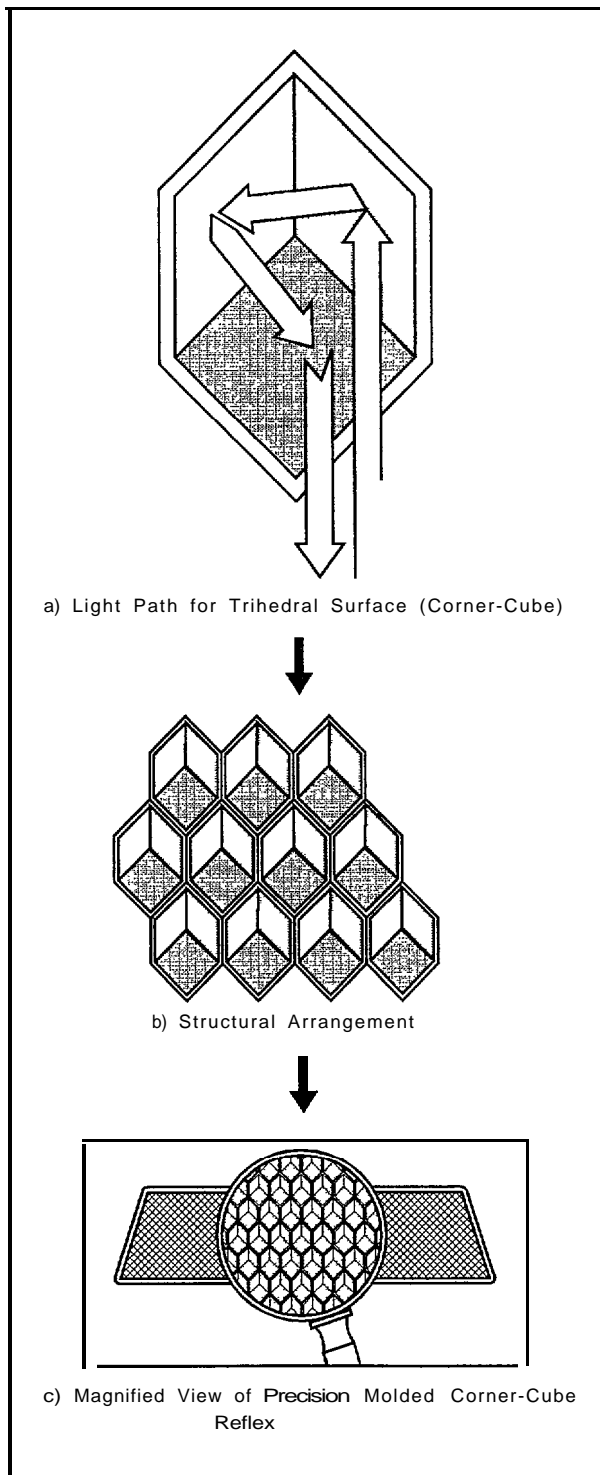
Figure 52. Principle and structure of corner-cube retroreflectors
