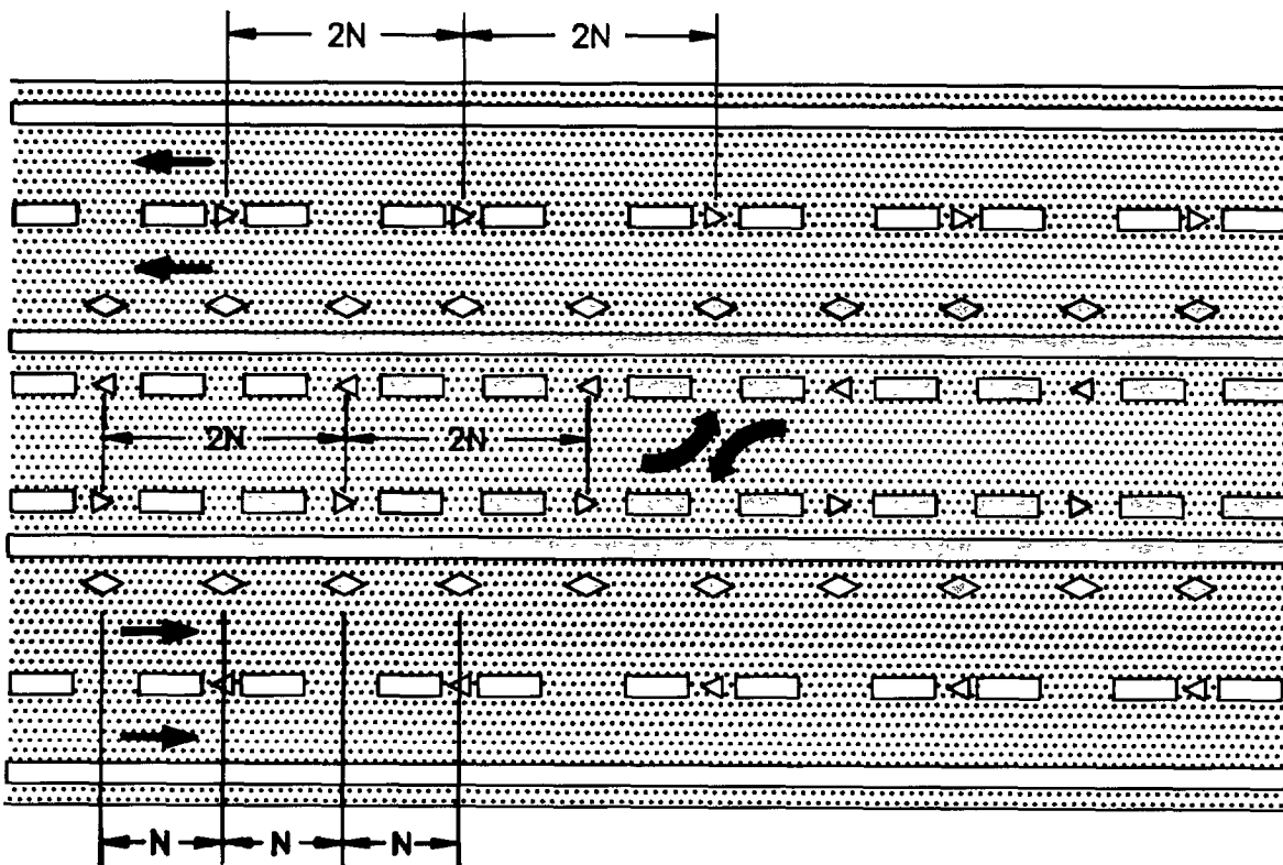
b) Center Lane of Five-Lane Road
