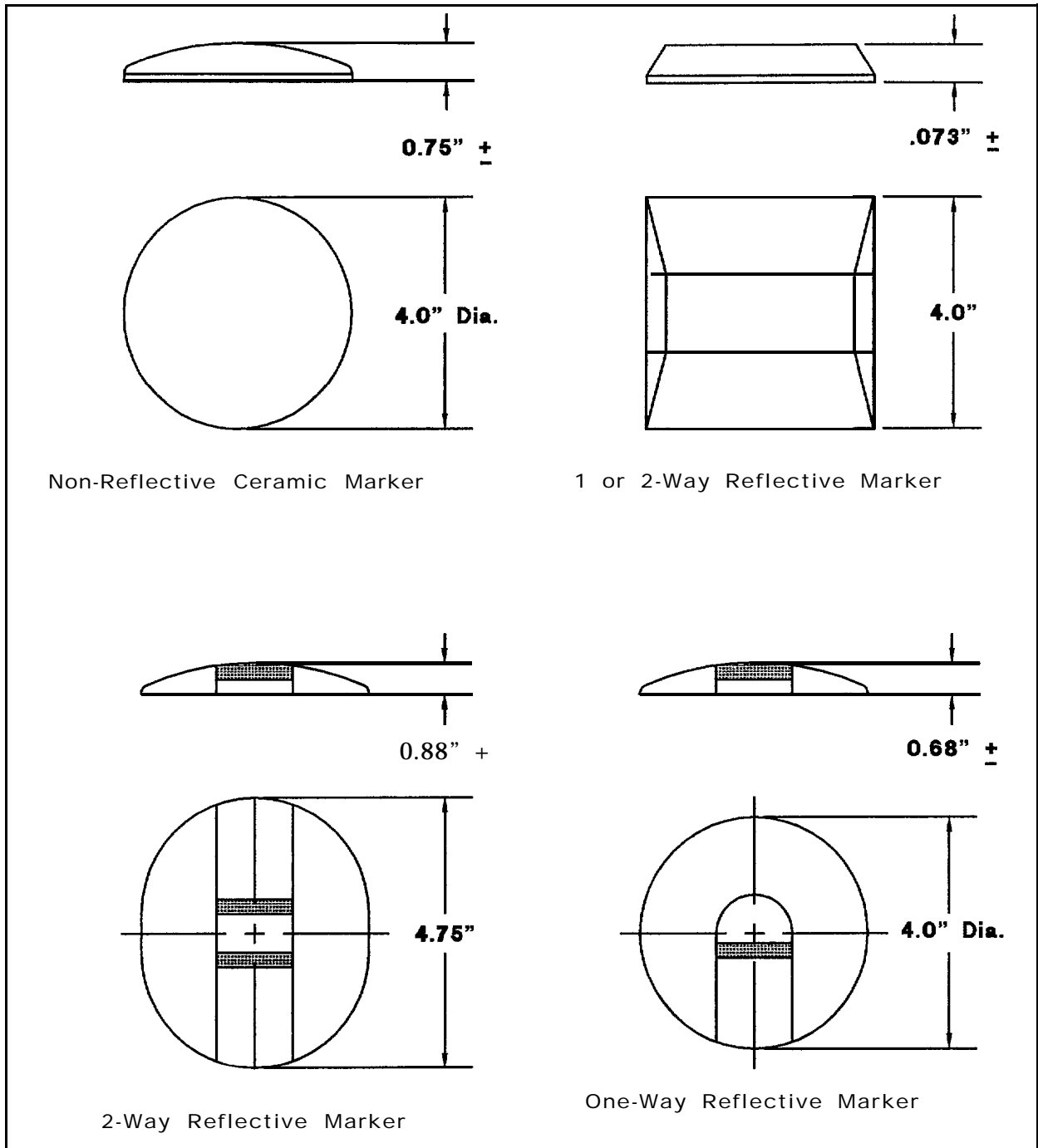
Figure 53. Typical raised marker configurations
