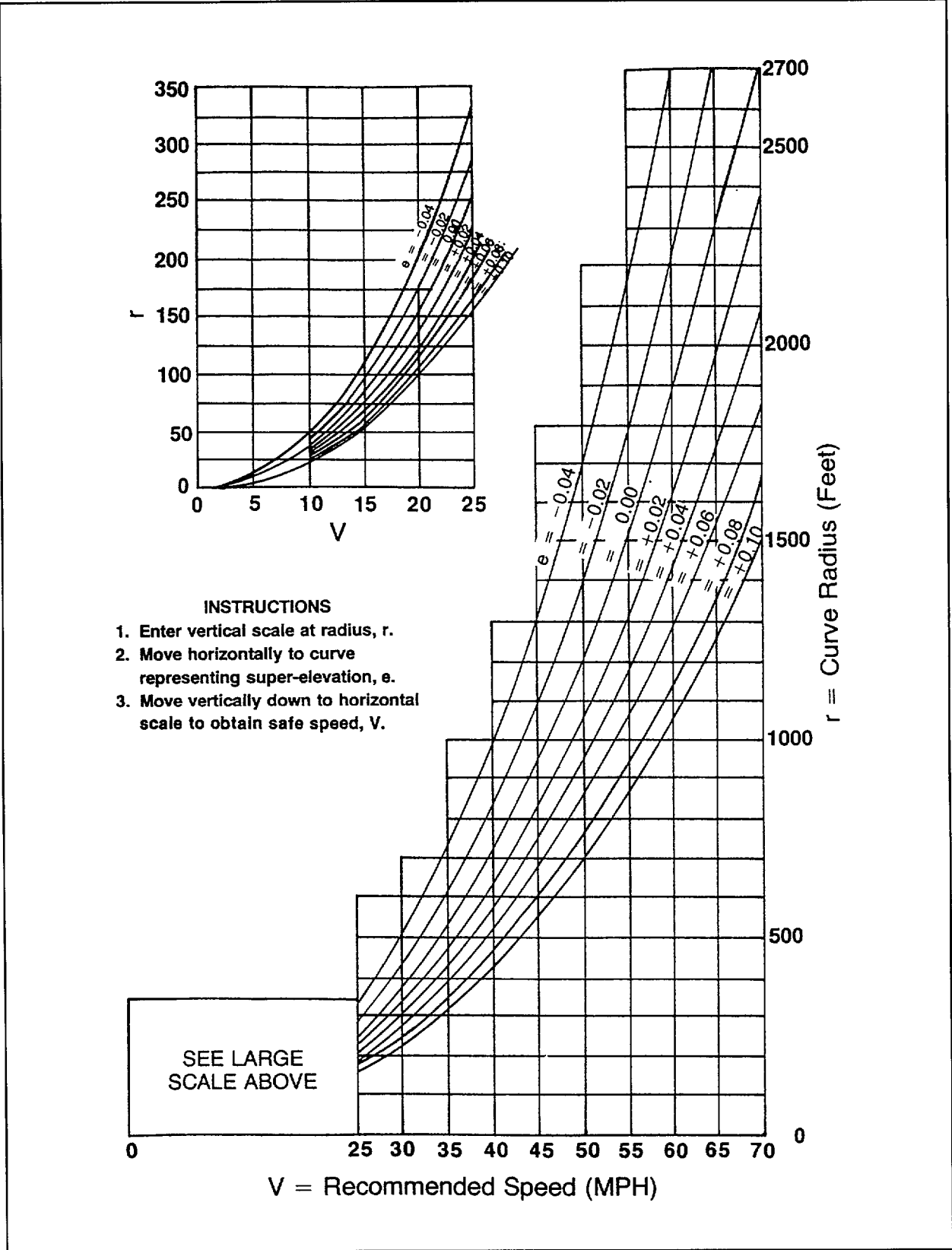
Figure 80. Recommended safe curve speed
