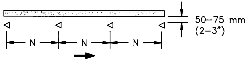
a) Combination RPM/Stripe for Left Edge Line (RPMs normally not recommended for right edge line)
