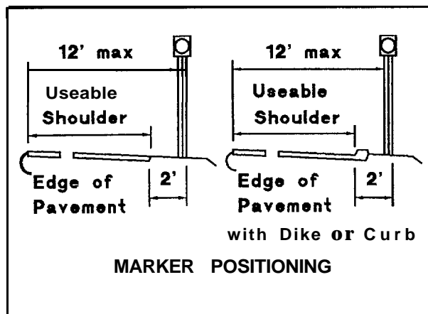
Figure 61. Typical delineator positioning
