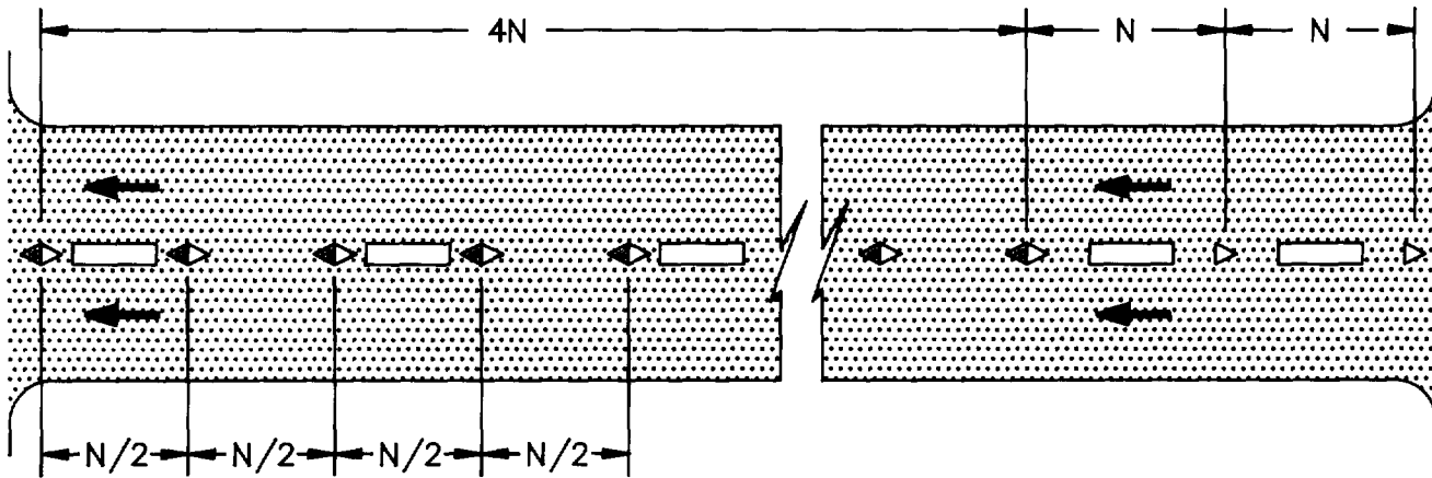
a) Two Lane, One-Way Road
