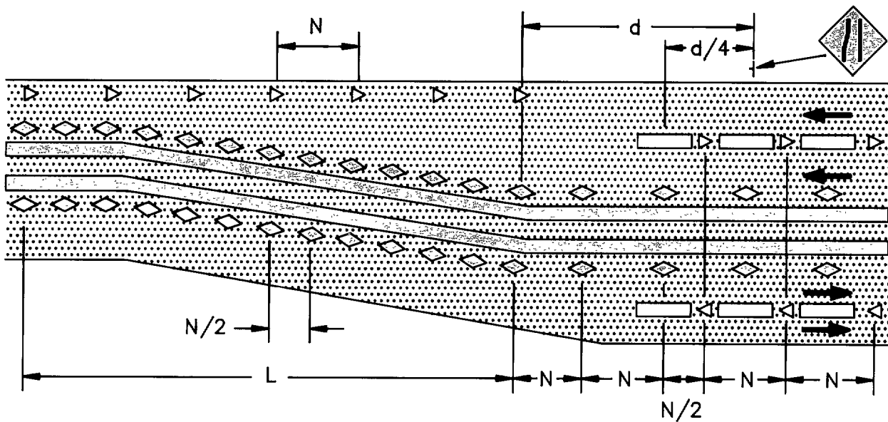
a) Four Lanes to Two-Lane Road - Right
