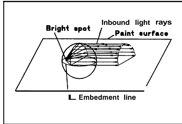
Figure 9. Focusing effect of glass beads
